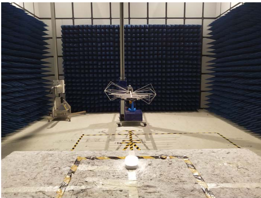
Photo 6 Test scene
